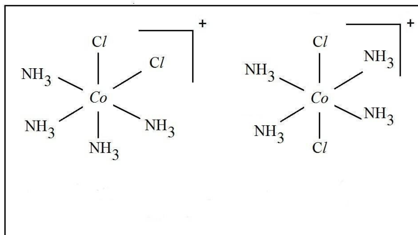
Fig 1b: Geometrical isomers (cis and trans) of [Co(NH_3)_4Cl_2] (Source: NCERT Textbook of Class 12 Chemistry, Page no. 251)
