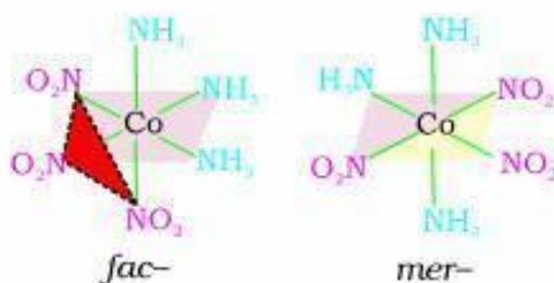
Fig 1d: The facial (fac) and meridional (mer) isomers of [Co(NH 3 ) 3 (NO 2 ) 3 ]
